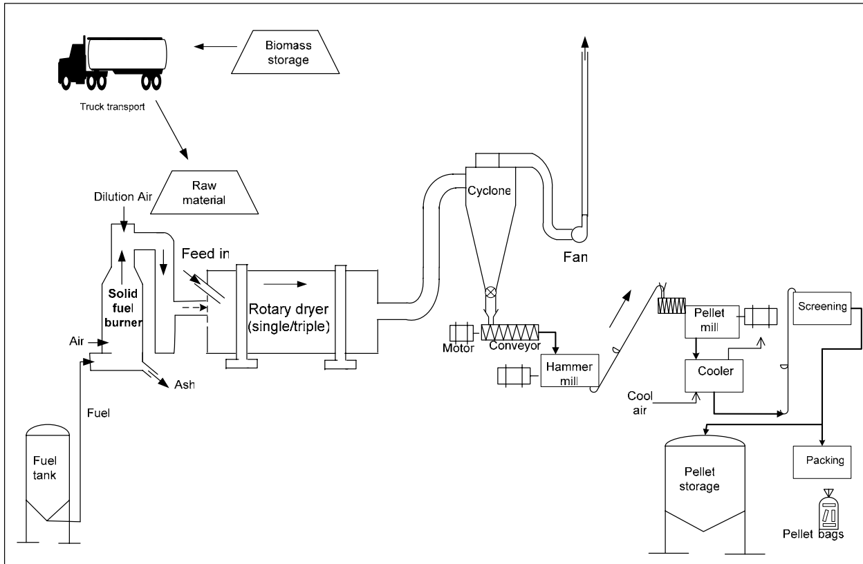
Figure C1. A schematic of pelletization plant used for cost analysis
